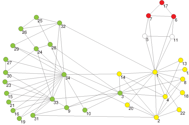
Figure 2: Zachary karate club communities after application of Rule 4.a (color online).
