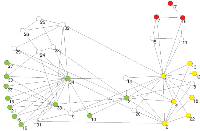
Figure 1: Zachary karate club communities after application of Rule 2; empty vertices are isolated at the current stage of resolution (color online).
