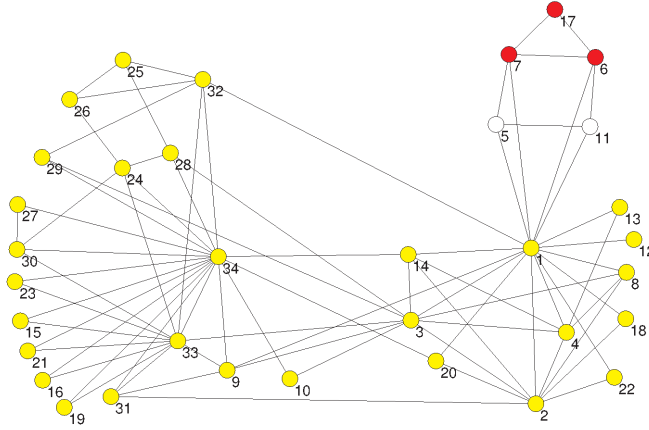
Figure 3: Zachary karate club communities after Rule 4.b (color online).
